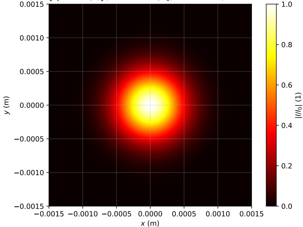
Intensity profile I(x, y, z = 0.478m)/I_0 , Pin=0.3Pcr, artificial time
